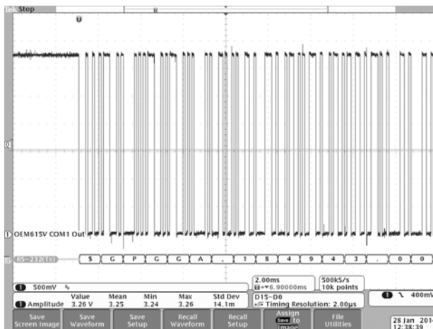
Figure 5: OEM719 COM1 output on CubeSat Kit Bus after OEM719 receives LOG COM1 GPGGA ONTIME 1 command. 15
